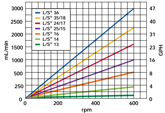
Flow Curves L/S® Easy-Load® II Pump Head
