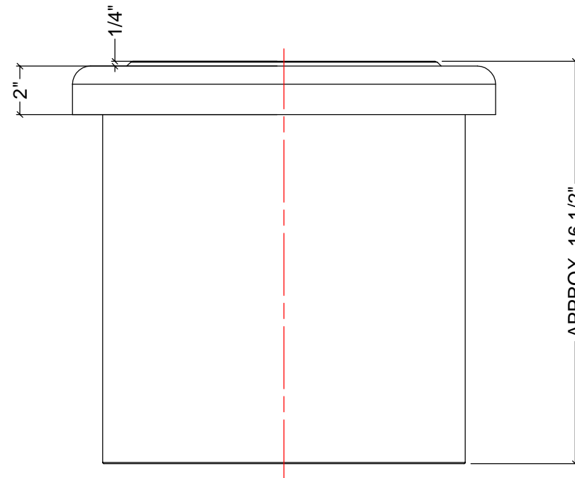
SIDE VIEW WITH LID
