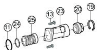
MECHANICAL SEAL END
