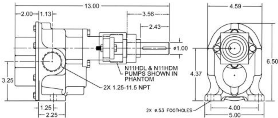
MECHANICAL SEAL END
